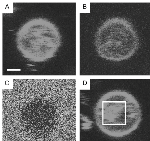
FIGURE 2 Giant vesicles in confocal microscope. Scale bar represents 1 \mu m. (A) Exciting Texas Red directly; imaging Texas Red emission. (B) The same vesicle under FRET, exciting FITC and imaging Texas Red, we see a weaker signal than direct excitation, as expected. (C): Exciting the FITC-labeled peptide reveals energy transfer to the TR-labeled membrane lipid as there is no increase in FITC signal along the GUV perimeter. (D) FRET of nested vesicle moving inside giant vesicle, suggesting that peptides can pass through the vesicle membrane.
