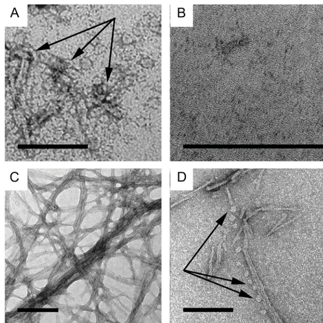
FIGURE 4 TEM images of soluble oligomers and fibrils \text{A}\beta_{1-40} . The scale bar represents 100 nm. (A) Soluble oligomers at the air-water interface. (B) Soluble oligomers in a lipid monolayer, structures are too small to see, but the stain is visible, indicating peptide presence. (C) Fibrils at the air-water interface, large three-dimensional networks are present. (D) With a lipid monolayer present, the mature fibrils are broken down into soluble oligomeric components.
