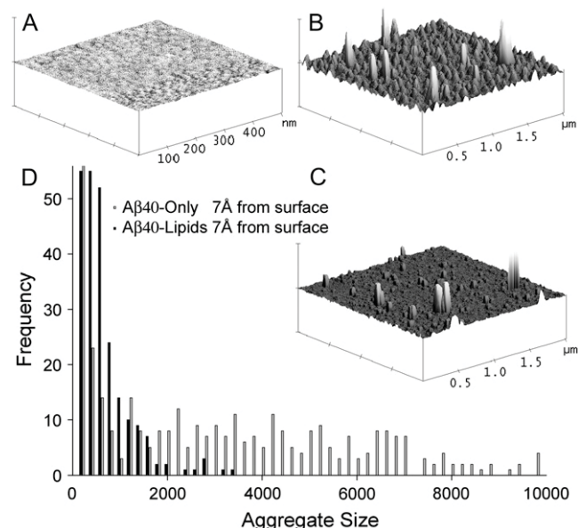
FIGURE 3 AFM height mode images. (A) Lipid monolayer 0.5 \mu\text{m} \times 0.5 \mu\text{m} 10-nm height scale reveals very small height undulations, indicating a fairly uniform monolayer. (B) \text{A}\beta_{1-40} without lipid monolayer reveals many high peaks. (C) Introducing the peptides into a lipid monolayer reduces the peak height and also peak width, in comparison to the system in panel B. (D) Aggregate size and size distribution, peptide with lipids, and peptide alone, the system with lipids induce a breakup of larger aggregates.
