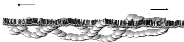
FIGURE 5 Proposed model for the fractionation of A \beta fibrils. The fibril consists of soluble oligomeric substructures; these come together to form a fibril because of hydrophobic interactions. The hydrophobic peptide segments preferentially incorporate into the hydrophobic tails of the monolayer lipids. Micro domains in the monolayer moving in different directions can tease the fibril apart, decomposing it into smaller fragments.
